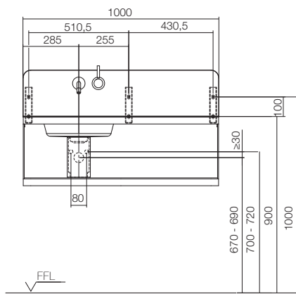
WP . S19L . 1 No. 5261 000 000
