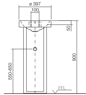
WT.RX400KH No. 4500 000 000 – with wall bracket cover
