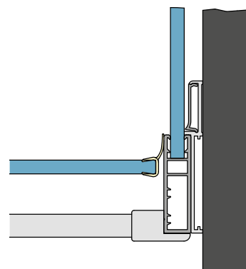
Detail A – pôdorys
